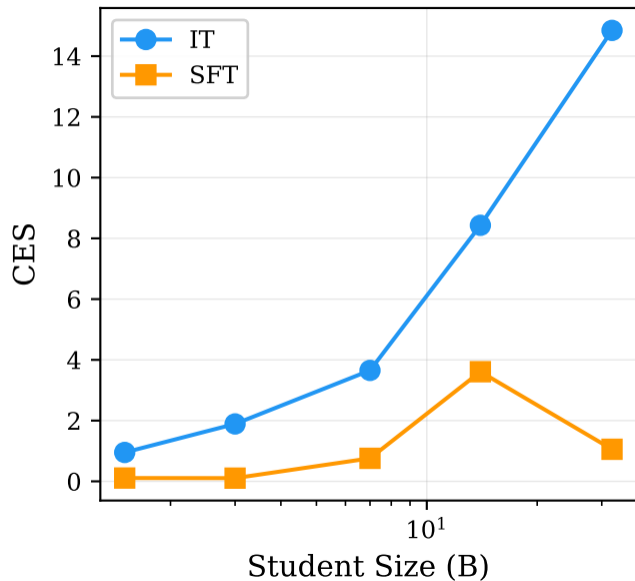
Compression Efficiency Score
