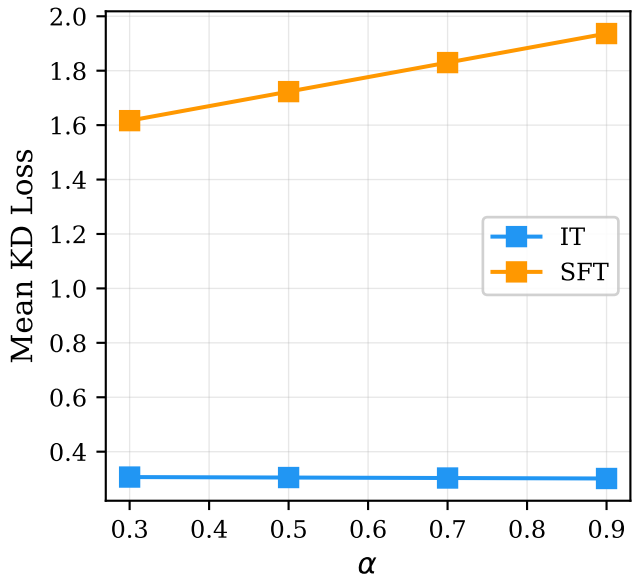
Loss vs. \alpha ( T = 2 )
