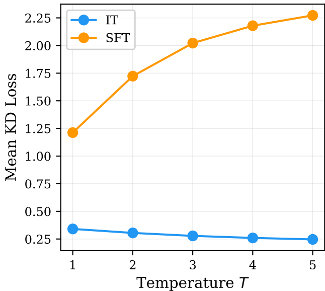
Loss vs. Temperature ( \alpha = 0.5 )
